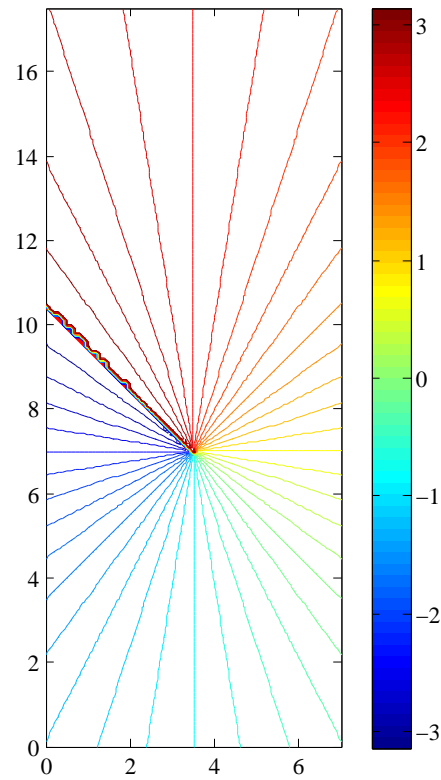
Figure 7.15: Contour plot of \theta of the slanted edge crack.
