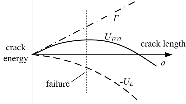
Figure 1.6: Energy changes of Griffith's problem
