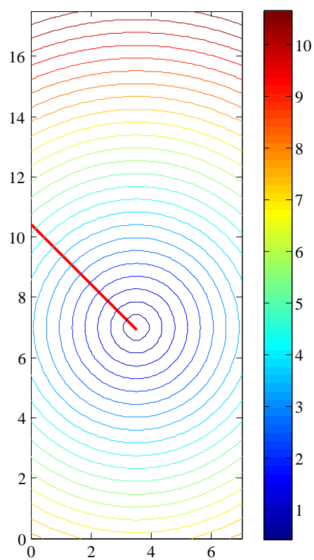
Figure 7.14: Contour plot of r of the slanted edge crack.
