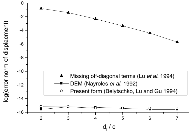
Figure 3.4: Displacement error norm with varying dI/c .
