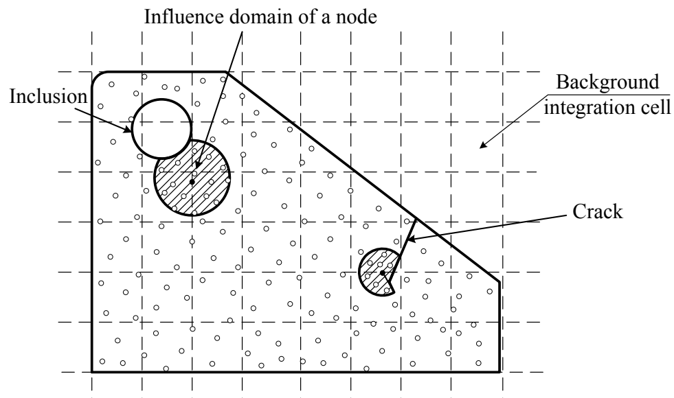
Figure 2.14: The background mesh used in the EFGM for integration. (reproduced from [3])
