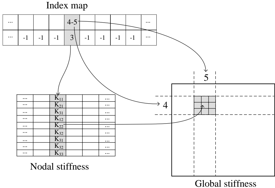
Figure 2.21: The vector storing nodal stiffness and the vector mapping nodal index to global stiffness position.
