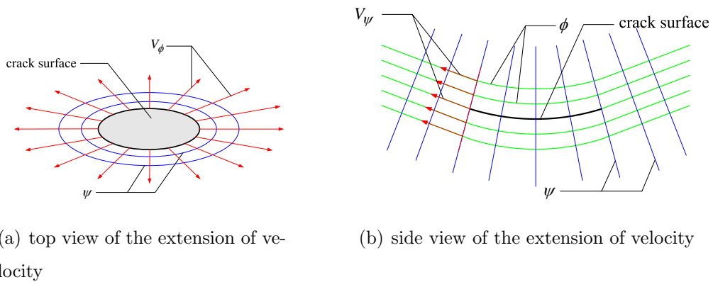
Figure 6.3: The extension of V_\phi and V_\psi along the orthogonal directions of \phi and \psi .
