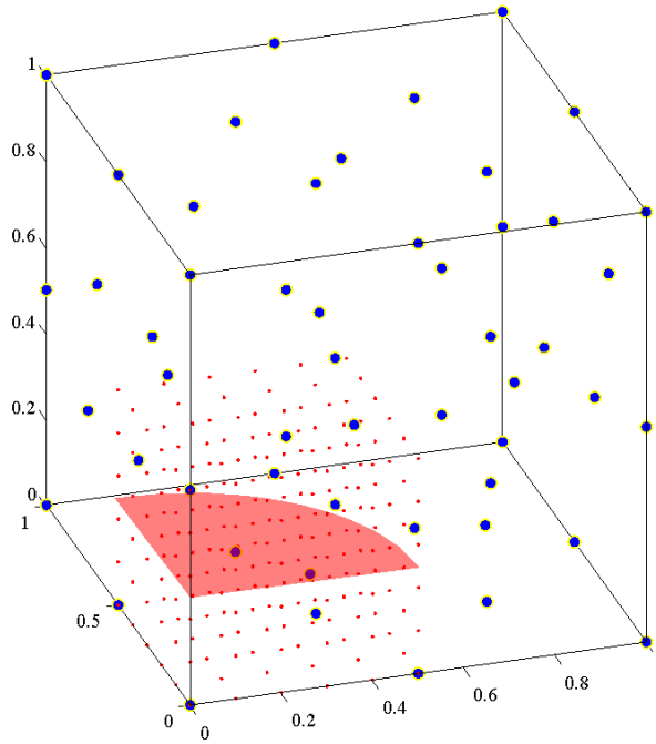
Figure 8.2: The structured level set grid decoupled from the meshless model.
