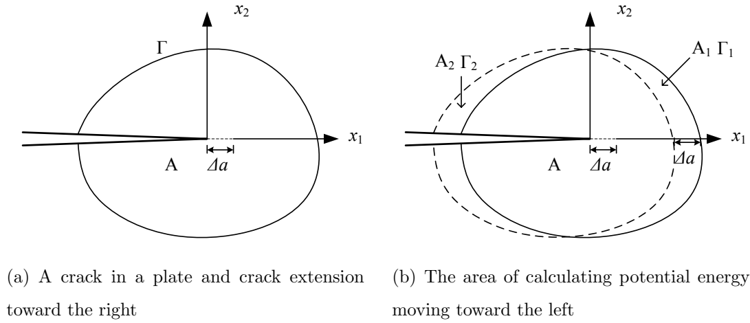
Figure 5.10: A 2D plate containing a crack and crack extension used for calculating potential energy.
