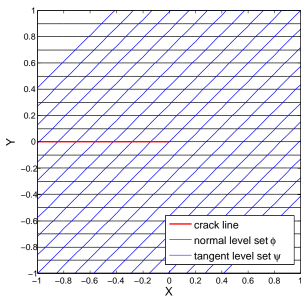
Figure 6.9: Level sets before reorthogonalization.
