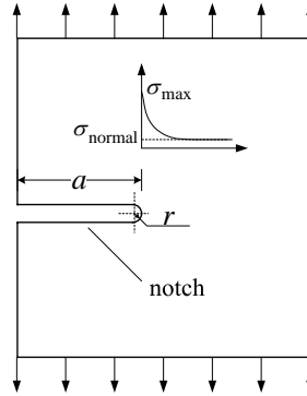
Figure 1.4: Stress concentration near a notch.
