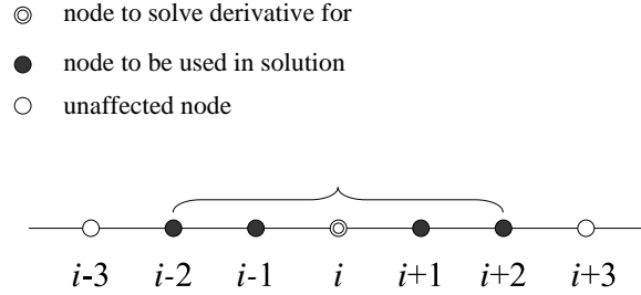
Figure B.1: The four neighbour points used to calculate the derivative at i .
