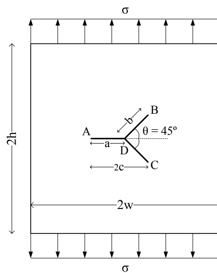
Figure 7.22: A symmetric branched crack in a finite plate under tension.
