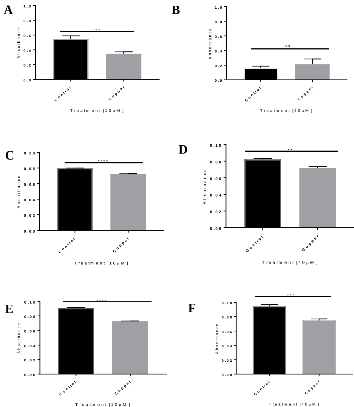
Figure 3.3: Exposure of CAD cells to sub-toxic (10 μM) and low-dose Cu (40 μM)- LDH
